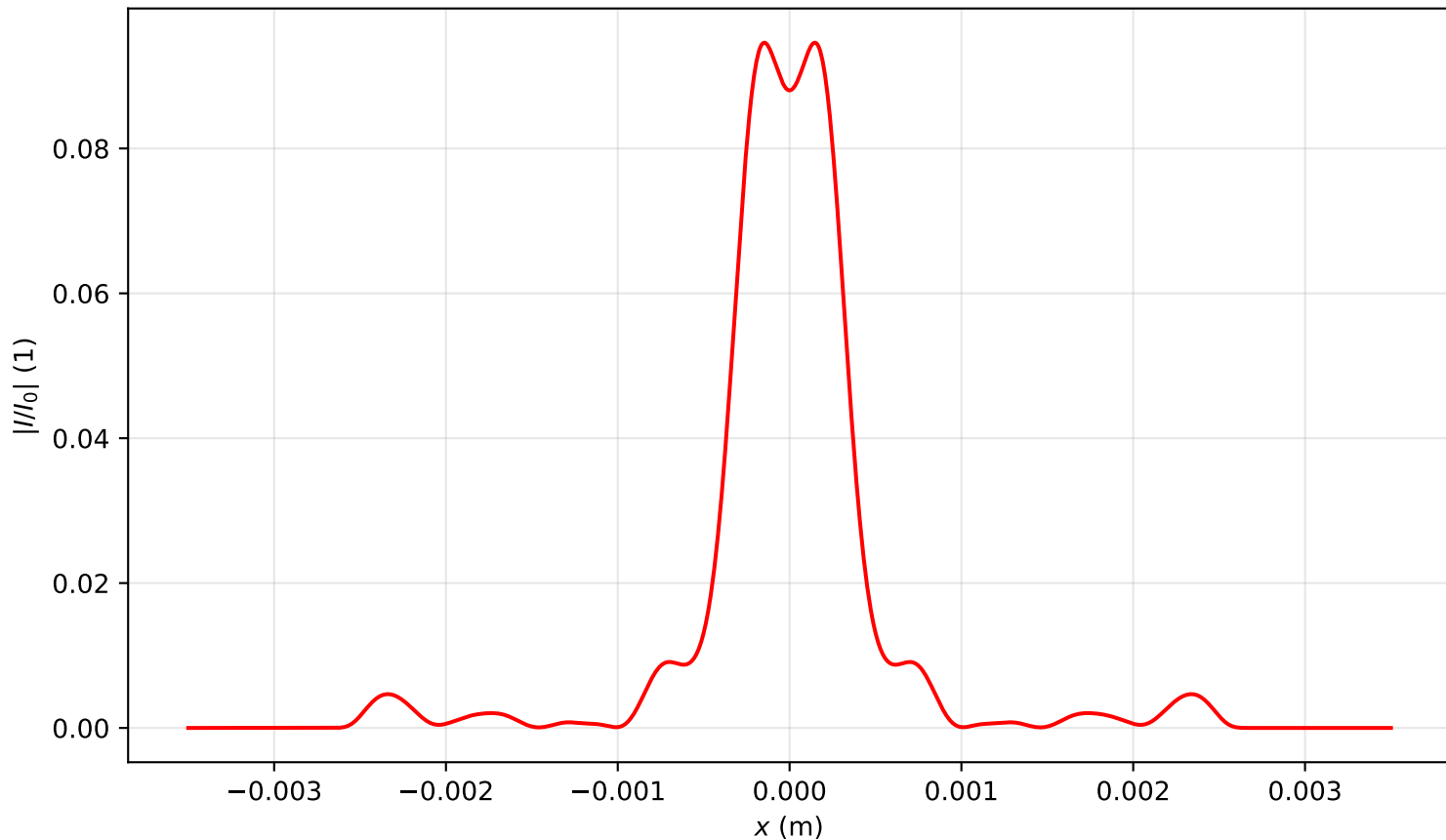
Intensity profile I(x, y = 0, z = 3.662)/I_0 , P_{in}=6.0P_{cr} , artificial time
